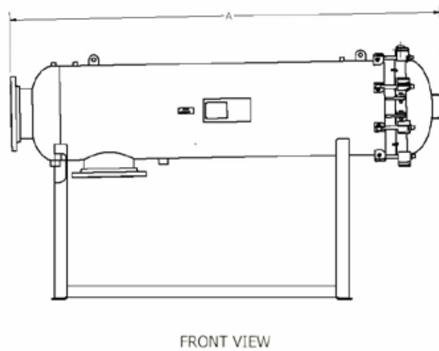
Figure 7: 3M™ High Flow 40"L & 60"L housings – Horizontal configurations
