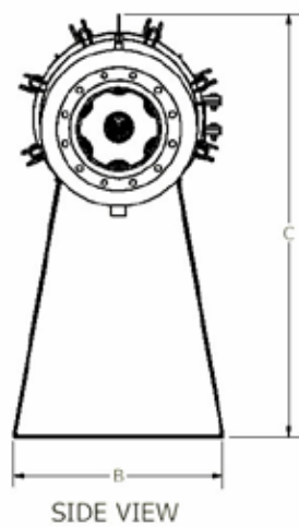
Figure 7: 3M™ High Flow 40"L & 60"L housings – Horizontal configurations
