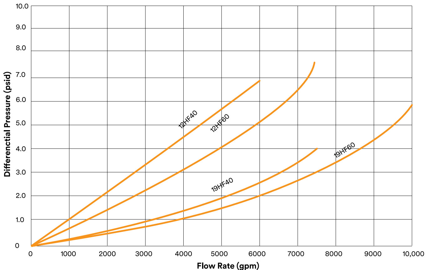
Figure 9: 3M™ High Flow housing (40"L &amp; 60"L) clean pressure drop vs. flow rates*
